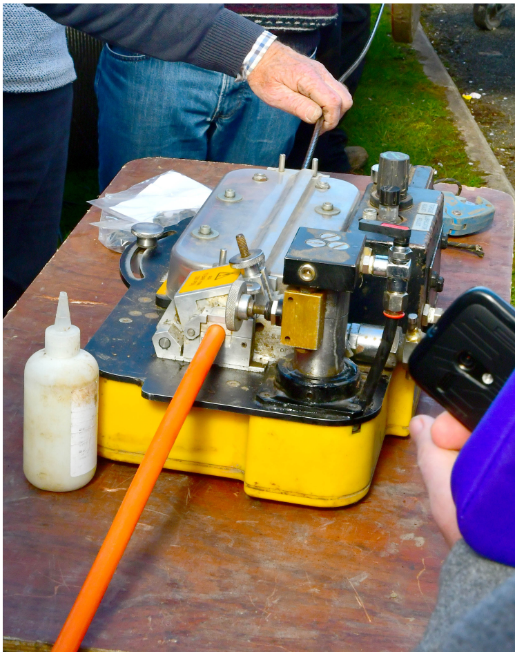
Blower used to send fibre down ducts
